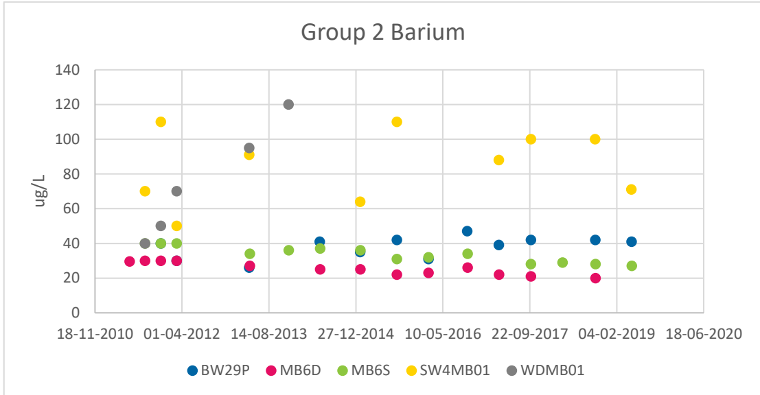
Figure 10-3 Group 2 Barium
