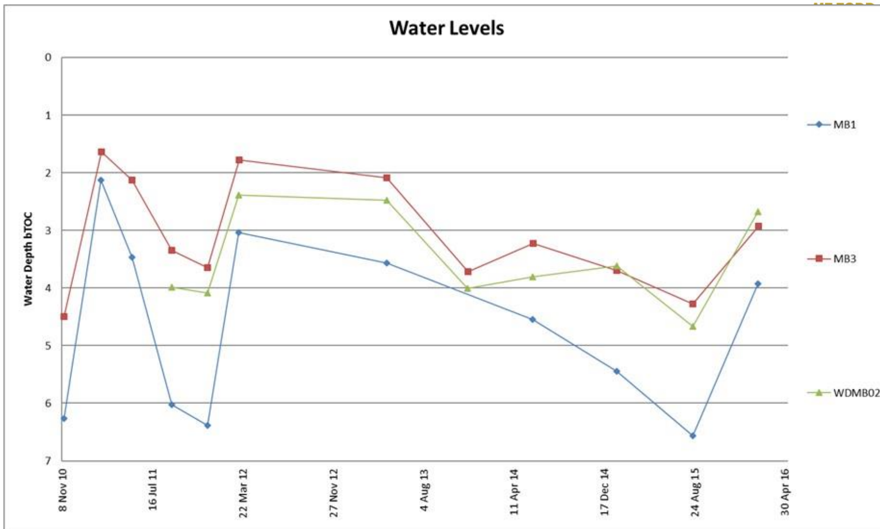
Figure 10-11 Group 2 Water Levels
