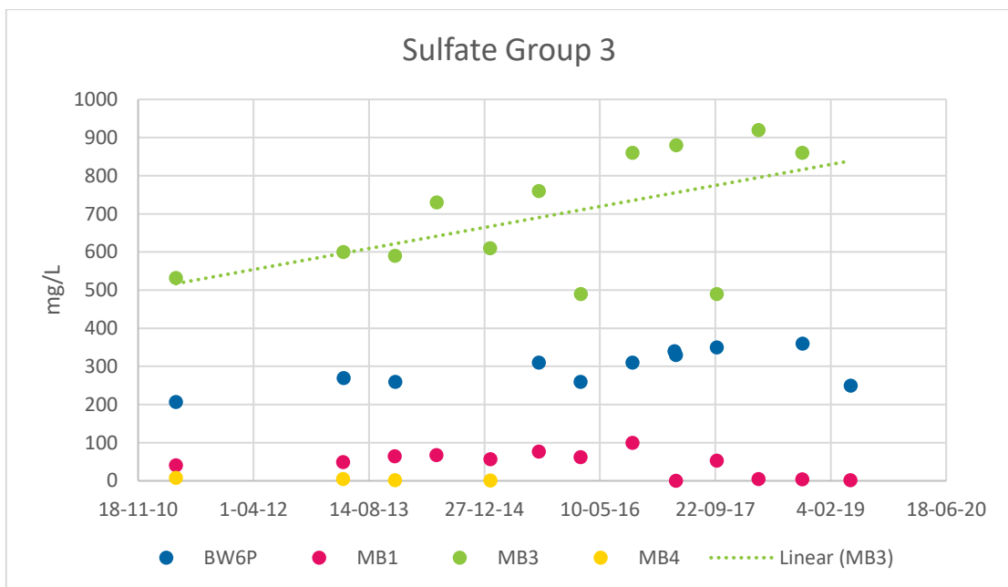
Figure 10-6 Group 3 Sulfate
