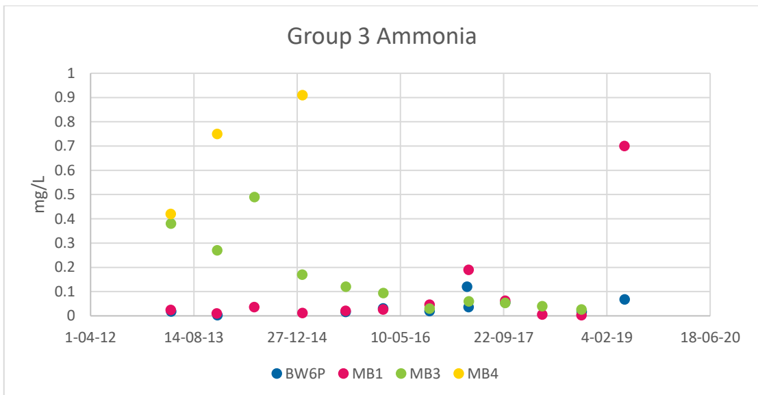
Figure 10-4 Group 3 Ammonia
